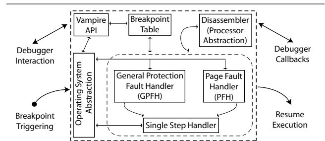
Figure 1. VAMPiRE Architecture
